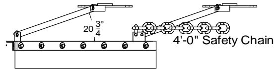
Position When Blades Are New
