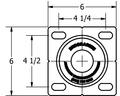
Mounting Bracket Dimensions
