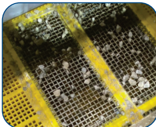
KNOCK DOWN STYLE HYBRID SCREEN PANEL
